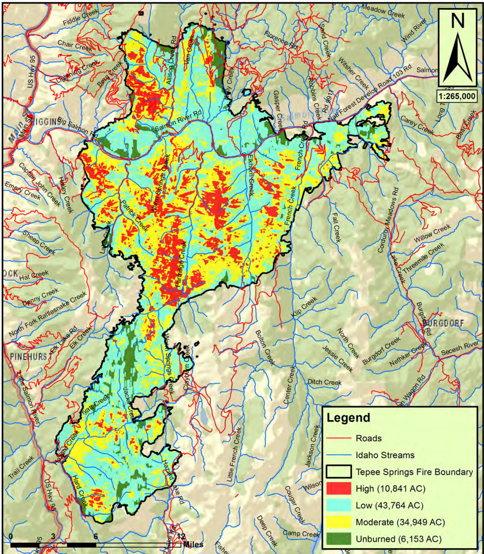
Burn Severity, Tepee Springs Fire
